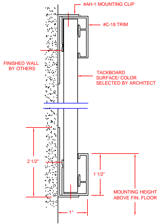
TACKBOARD
