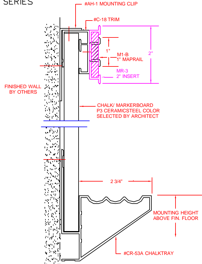
CHALK/ MARKERBOARD
